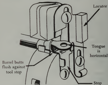
FIGURE 4-107. Inserting terminal lug into hand tool.
